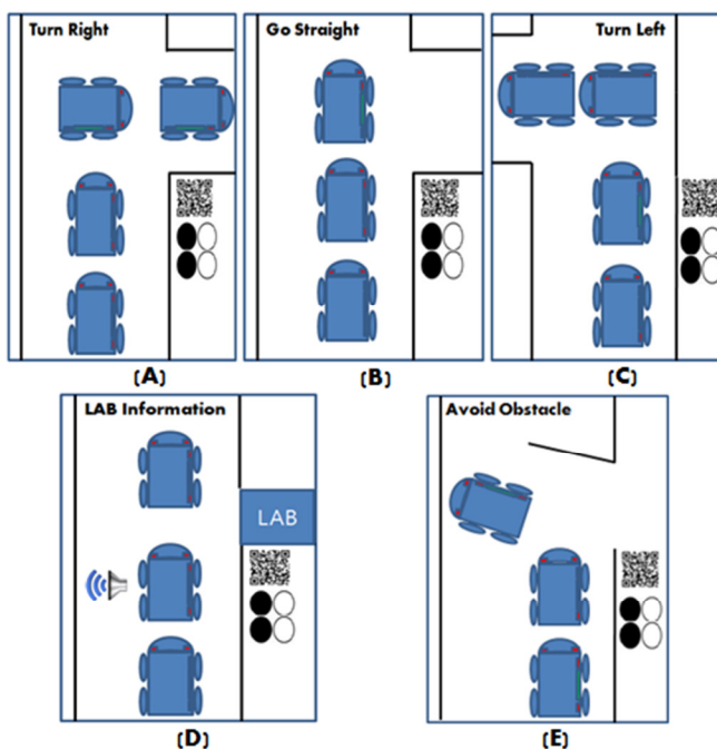
Fig. 6. Information obtained from QR code recognition helps to aid autonomous robot motion. The information in QR code is stored as follows. (A) Turn Right, (B) Go Straight, (C) Turn Left, (D) LAB Information, and (E) Avoid Obstacle.
